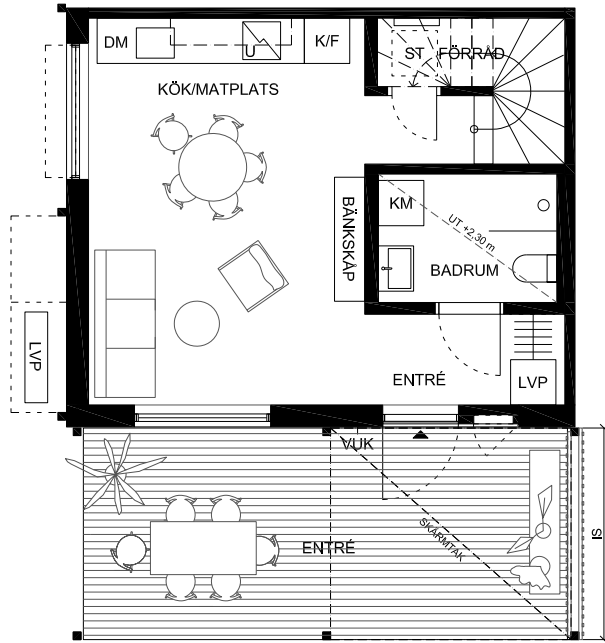
MARKPLAN
