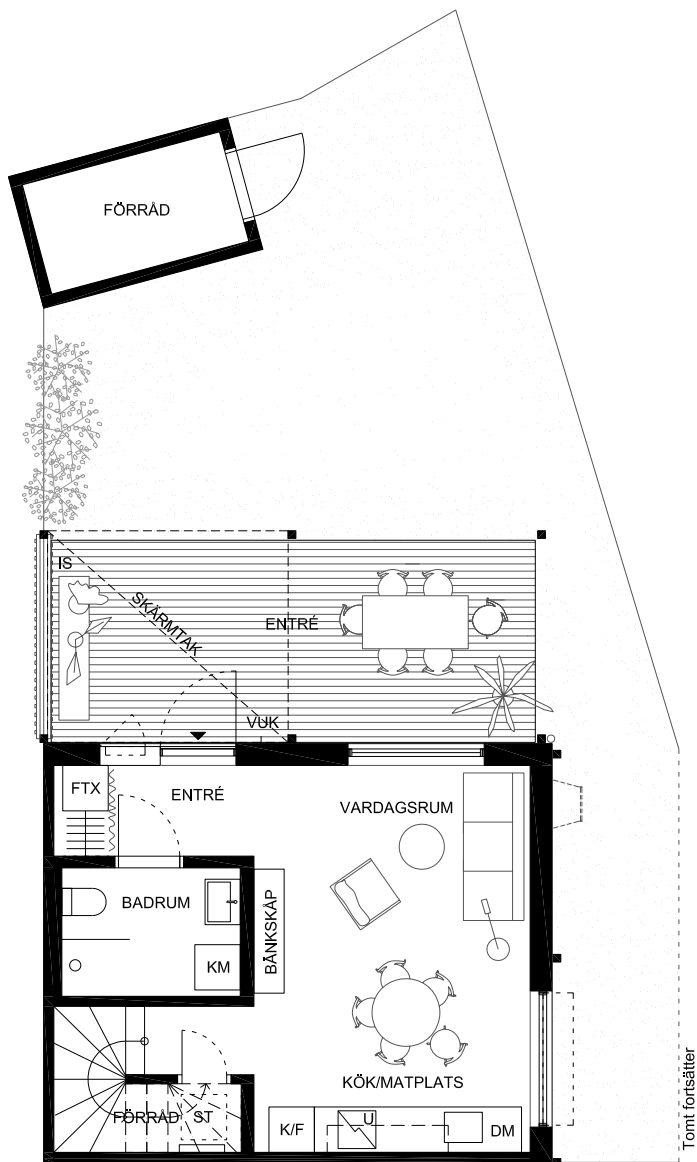
MARKPLAN
